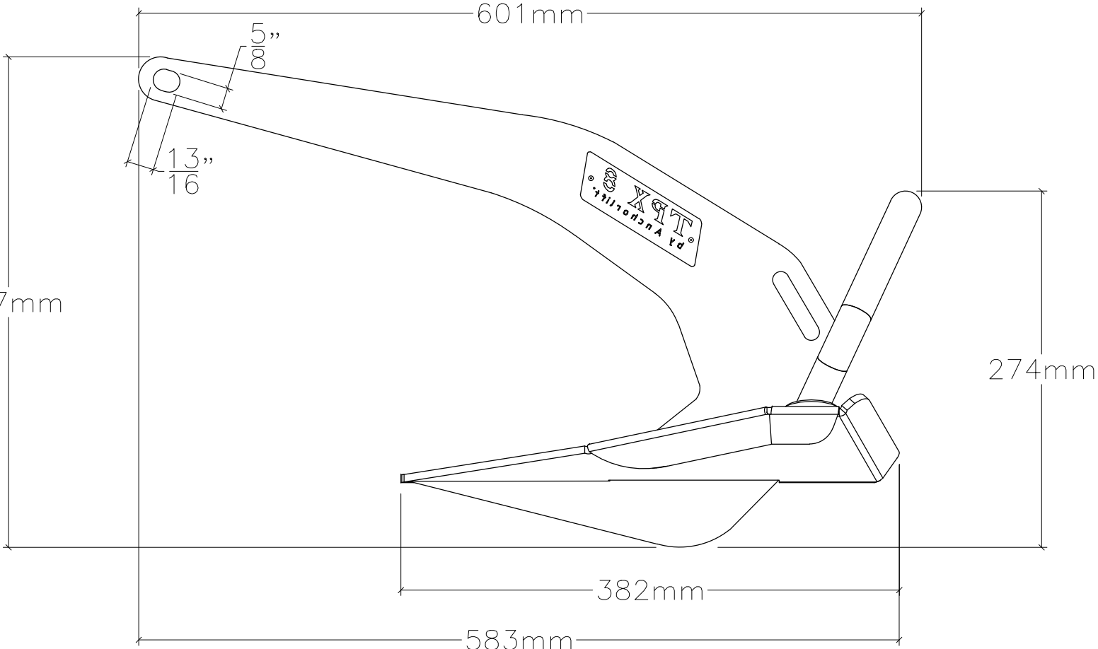
SIDE VIEW
