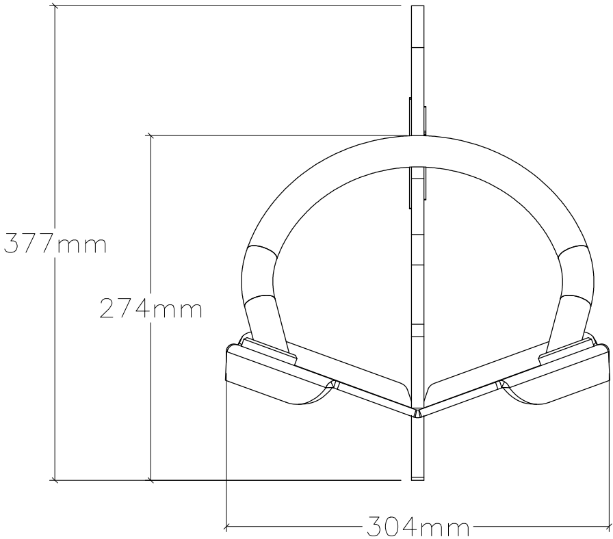
FRONT VIEW
