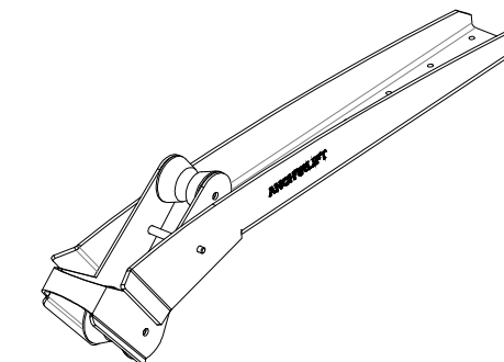
3-D VIEW
