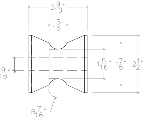
ROLLER #1
