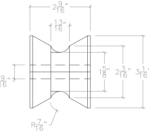
ROLLER #2
